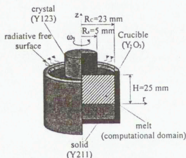
Fig.1 Schematic diagram
