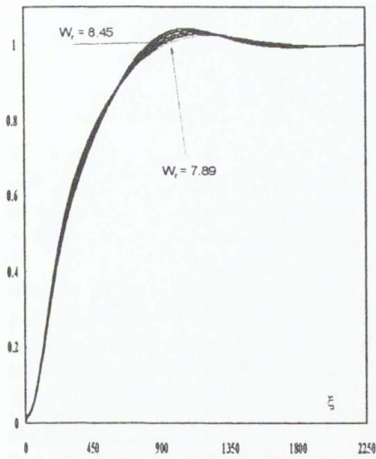
Fig.5 Capillary shock waves for \alpha = 15 .
