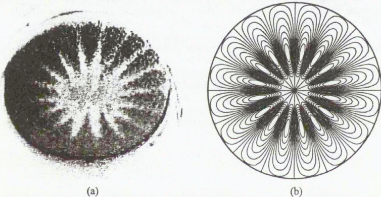
Fig.2. (a) Photograph of temperature field taken at the horizontal cross-section z = 0.95H , Gr \approx 2.5 \times 10^4 (from [1]); (b) Isolines of perturbation of temperature at the cross-section z = 0.95A (from [2]).
