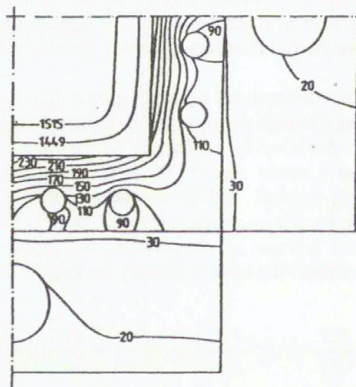
Figure 2. The calculated temperature field in the blank, the crystallizer and in the frame in a cross-section led
