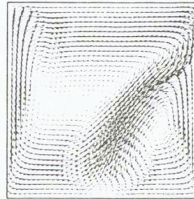
Numerical simulation adiabatic walls. Stream function (left), velocity field (right)
