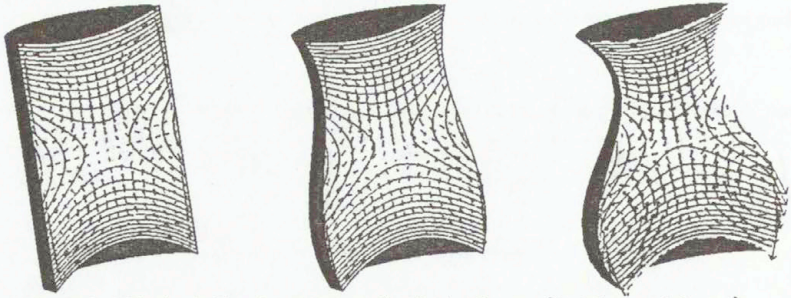
Figure 2. Velocity field and temperature distribution for g \in \{0, 1.0 * g_E, 2.0 * g_E\}
