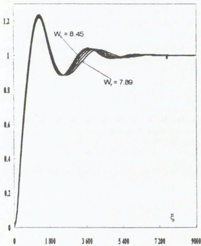
Fig.7 Capillary shock waves for \alpha = 50 .
