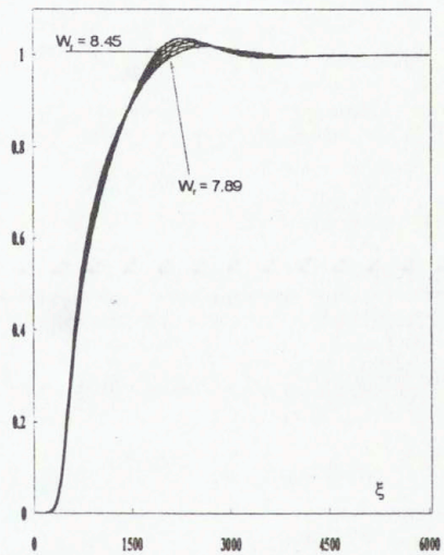
Fig.8 Kinetic shock waves for \alpha = 50 .
