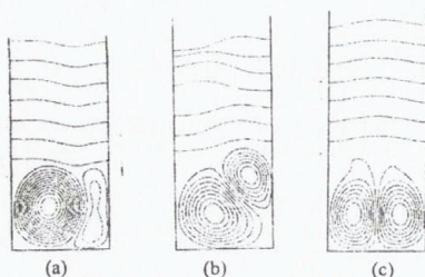
Figure 2. Interface shape for Ra = 10^5 ; (a) k_s/k_l = 2 , (b) k_s/k_l = 1 and (c) k_s/k_l = 1/2 .
