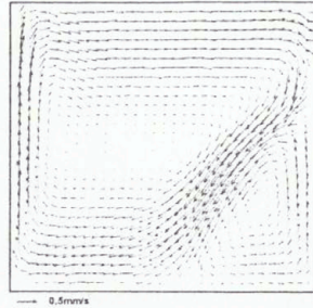
Natural convection velocity field (PIV)
