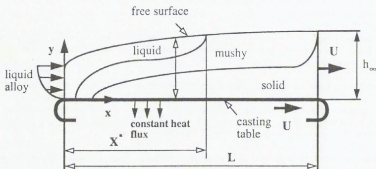
Figure 1. Definition sketch
