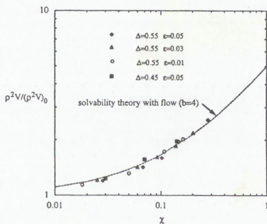
Figure 2. Predicted ratio of the selection constant p^2V with flow to without flow as a function of the dimensionless flow parameter \chi and comparison with microscopic solvability theory 3
